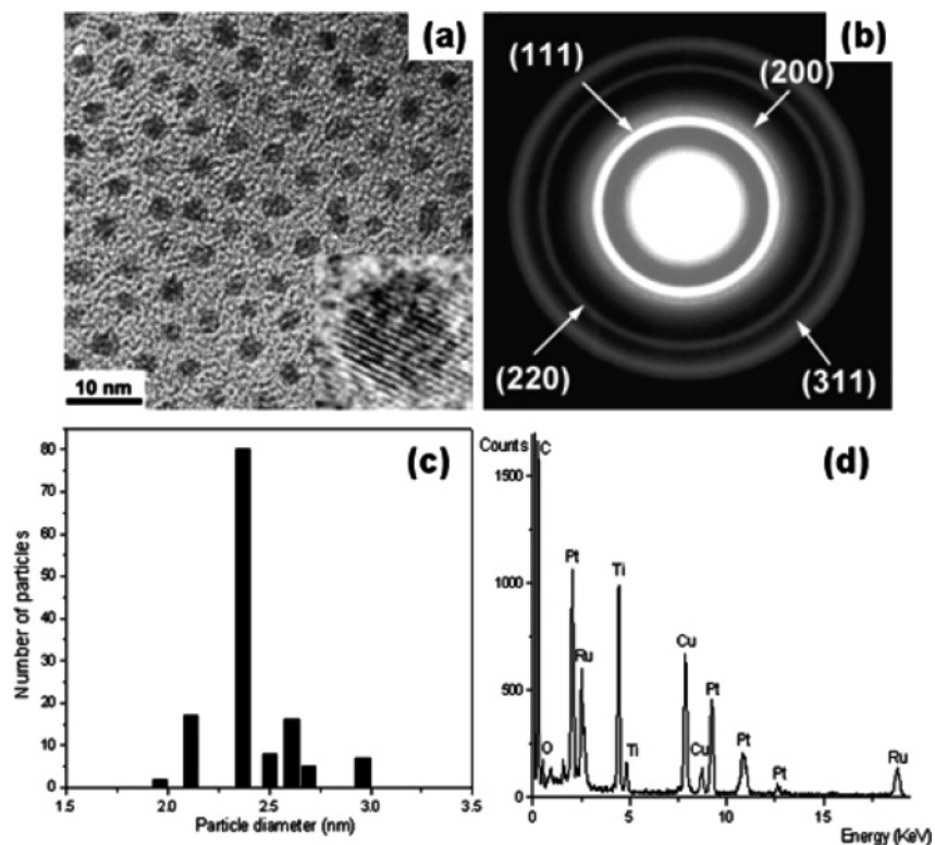
Figure 1. (a) TEM image of the colloidal PtRu nanoalloy (the inset represents the HRTEM image). (b) Selected area electron diffraction pattern. (c) Histograms of the particle distributions for colloidal PtRu nanoalloy as measured from 180 particles in TEM micrographs. (d) Typical EDX spectrum of colloidal PtRu nanoalloy.
