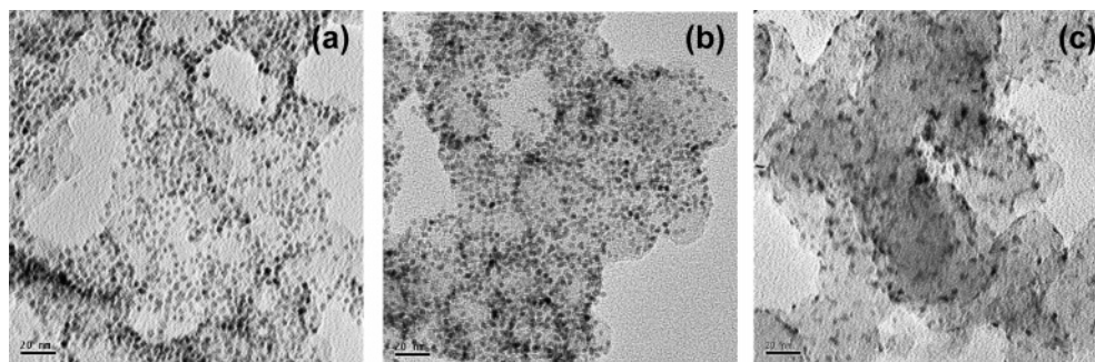
Figure 2. TEM images of (a) colloidal PtRu/Vc catalyst precursor, (b) PtRu/Vc catalyst, and (c) commercial E-TEK catalyst.
