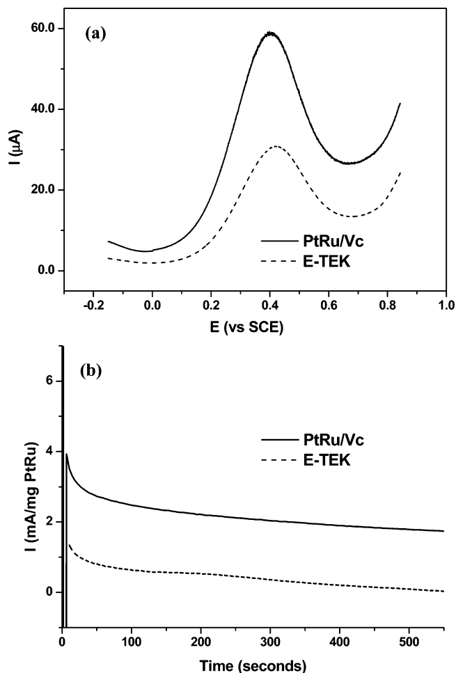
Figure 3. (a) Linear sweep voltammograms (scan rate = 0.010 V/s) and (b) chronoamperometry measurements of methanol oxidation in 1 M CH 3 OH and 0.05 M H 2 SO 4 solution for an electrode coated with PtRu/Vc catalyst (solid line) and with commercial E-TEK catalyst (dashed line).
